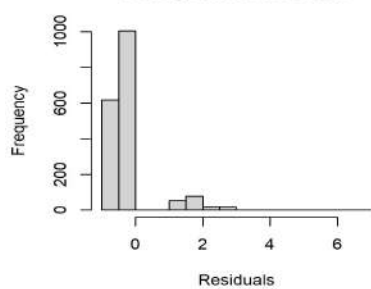
Histogram of residuals
