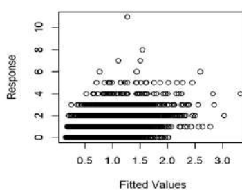
Response vs. Fitted Values
