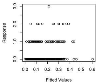
Response vs. Fitted Values
