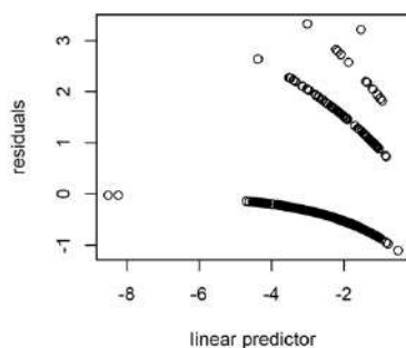
Resids vs. linear pred.
