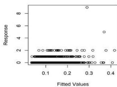
Response vs. Fitted Values
